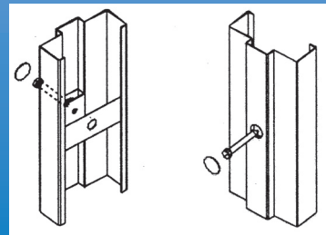
Concealed EMA with Caps
