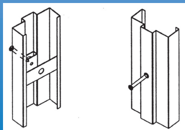
EMA Pierce & Dimple
