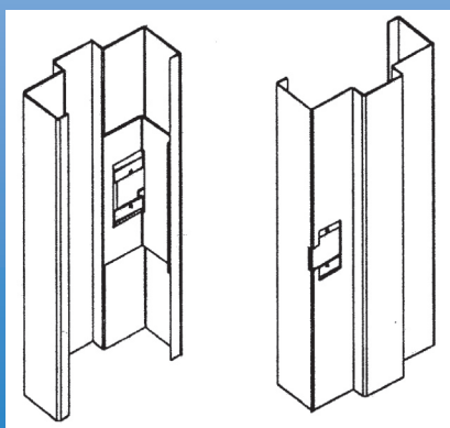
12 Gauge Strike Reinforcement
