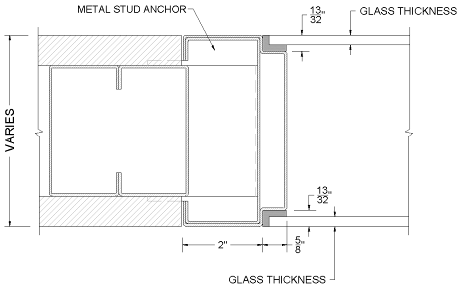
Jamb/Head Sill Detail
